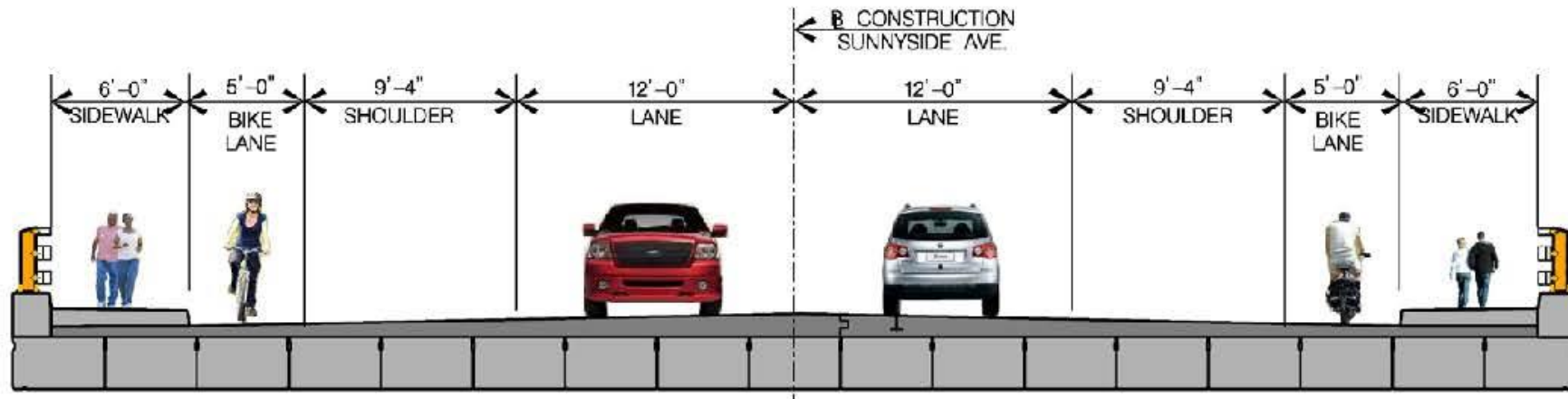
PROPOSED BRIDGE
